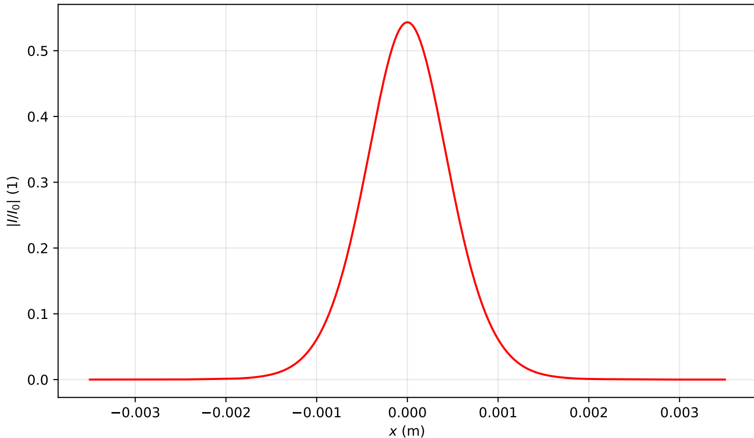
Intensity profile I(x, y = 0, z = 3.105)/I_0 , P_{in}=0.5P_{cr} , artificial time
